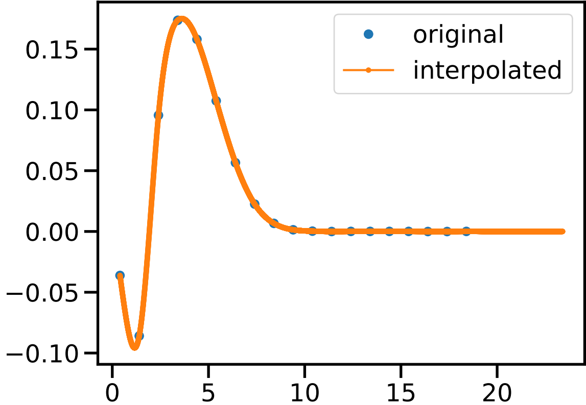
Hamiltonian Interpolation After Training (14, 14, 0, 2)
